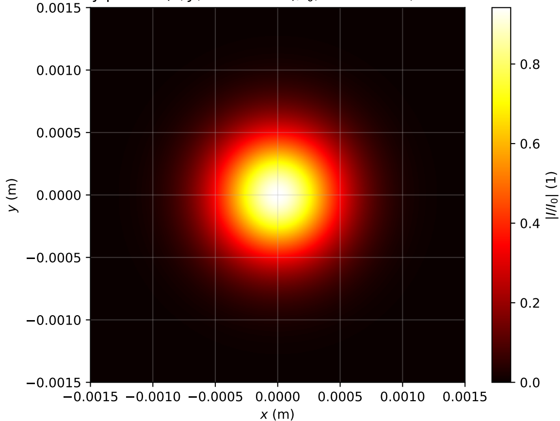
Intensity profile I(x, y, z = 0.955m)/I_0 , Pin=0.3Pcr, artificial time
